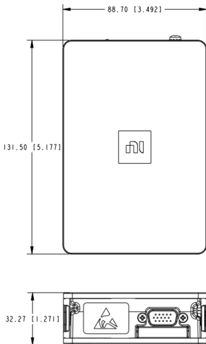
Figure 1. cDAQ-9170 Dimensions
