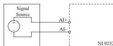
Figure 5 : Connecting a Floating Signal Source
