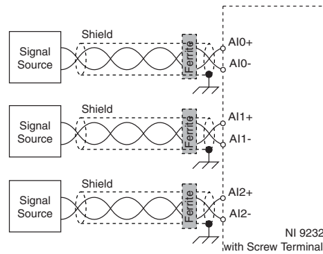
Figure 3 : Cable Connections for EMC Compliance
