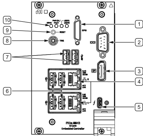
Figure 2. PXle-8842 Front Panel Layout
