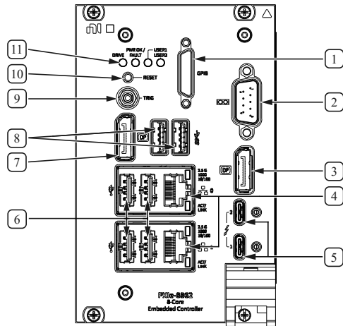
Figure 3. PXle-8862 Front Panel Layout
