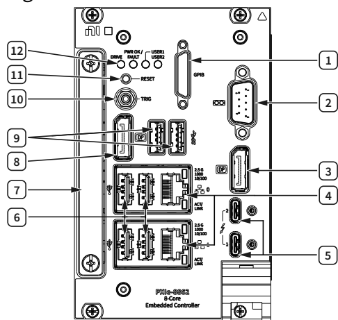
Figure 4. PXle-8862 with Removable Hard Drive Front Panel Layout
