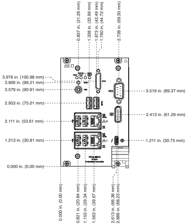
Figure 6. PXle-8842 Front Panel Layout and Dimensions
