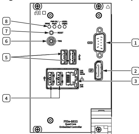
Figure 1. PXle-8822 Front Panel Layout
