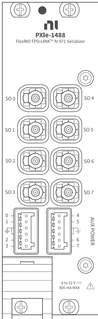
Figure 3. Serializer Front Panel
