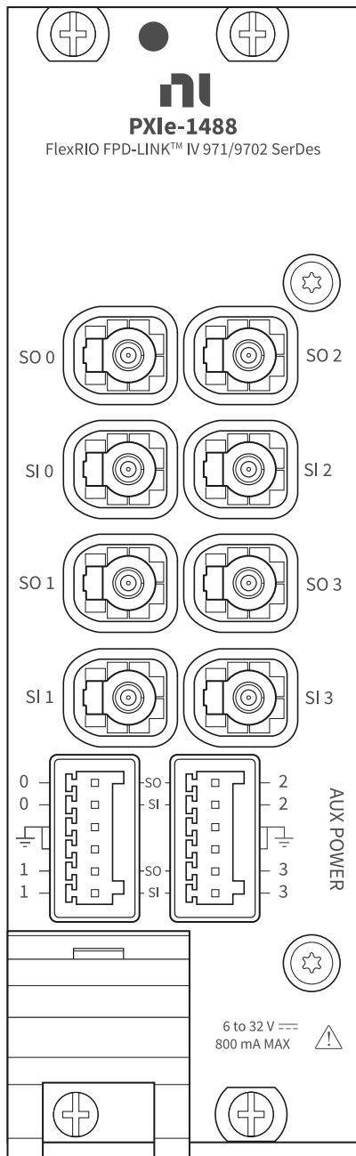
Figure 5. SerDes Front Panel
