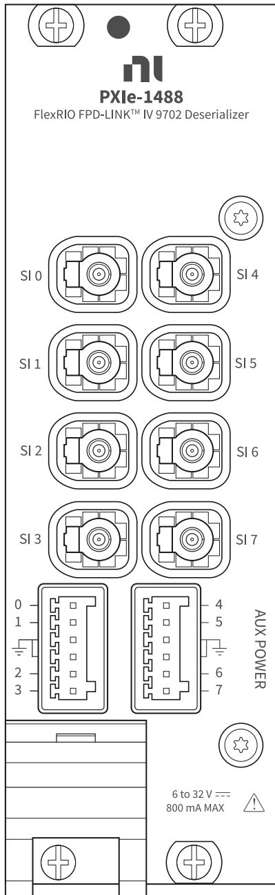
Figure 1. Deserializer Front Panel
