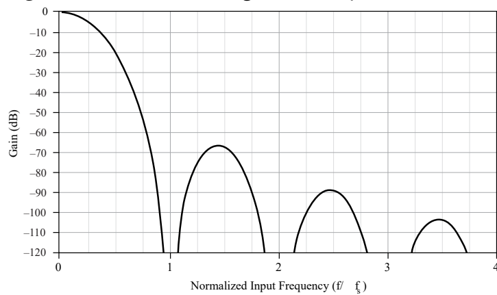
Figure 10. Comb Filter Magnitude Response
