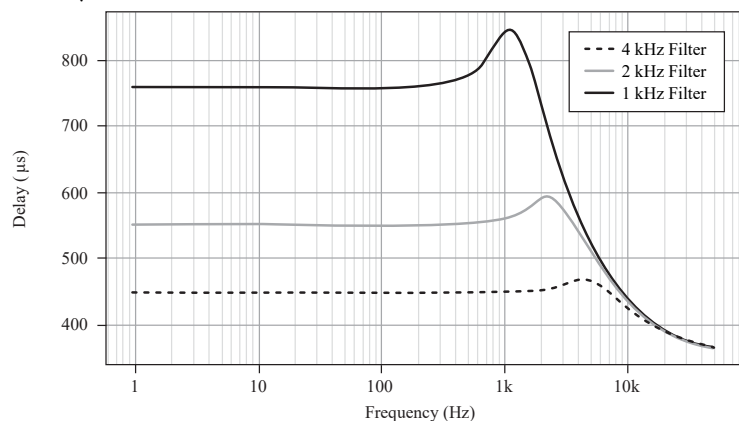
Figure 8. Butterworth Filter Input Delay (4th Order, with 12.8 MHz Timebase, 500 Hz, 250 Hz, 125 Hz Filter)
