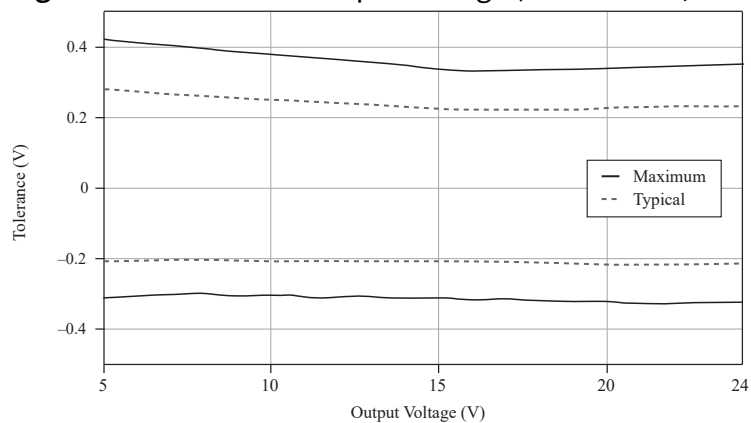
Figure 1. Tolerance vs Output Voltage (5 °C to 40 °C, 1 mA Output)
