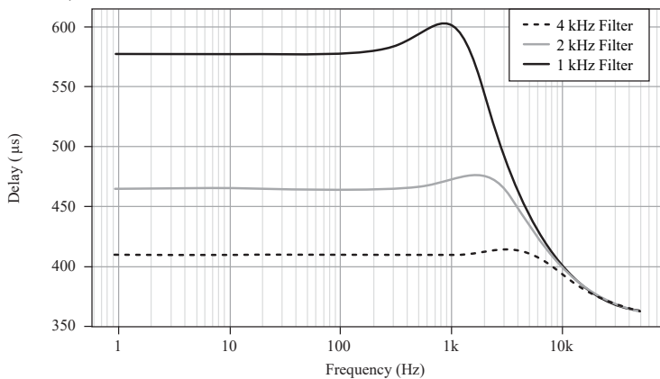
Figure 6. Butterworth Filter Input Delay (2nd Order, with 12.8 MHz Timebase, 500 Hz, 250 Hz, 125 Hz Filter)
