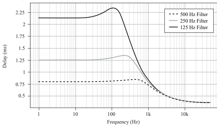
Figure 7. Butterworth Filter Input Delay (4th Order, with 12.8 MHz Timebase, 4 kHz, 2 kHz, 1 kHz)
