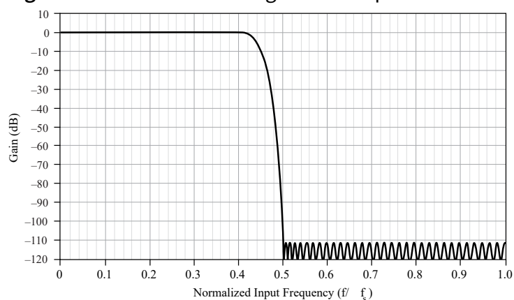
Figure 4. Brickwall Filter Magnitude Response
