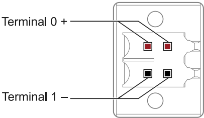
Figure 6. PXle-4113 Auxiliary Power Input Connector
