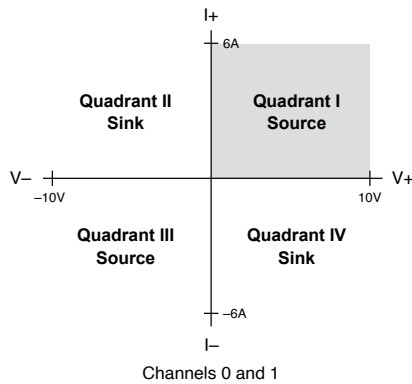
Figure 7. PXle-4113 Quadrant Diagram
