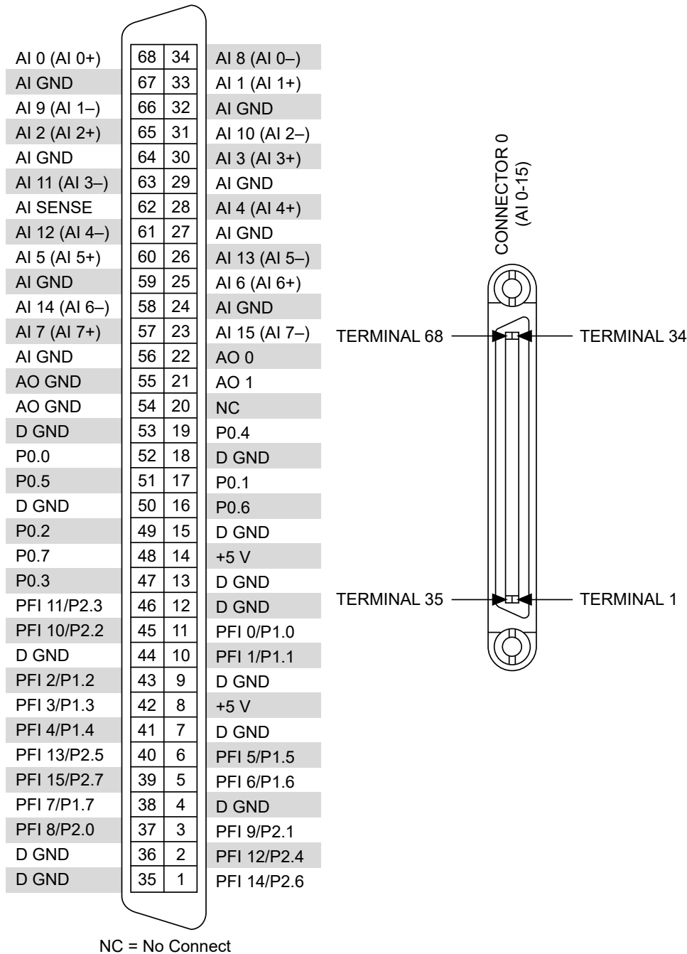
Figure 1. PXle-6321 Pinout
