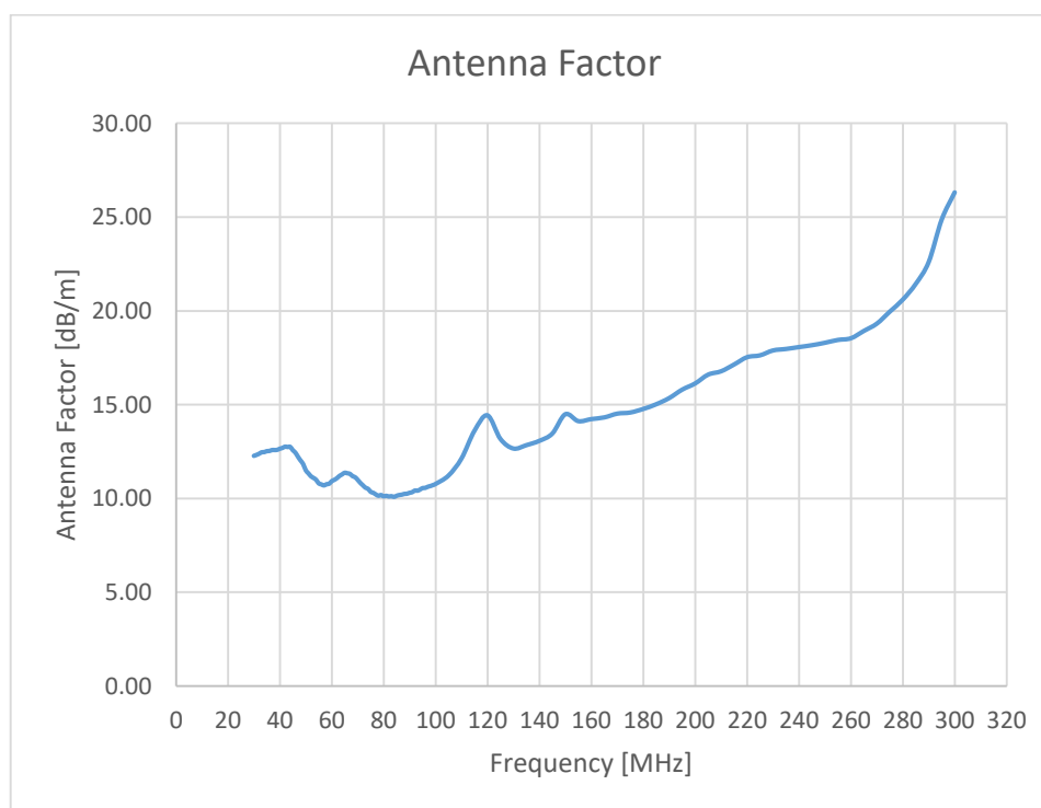
Figure 3: TBMA2 Antenna Factor (30 MHz...300 MHz)
