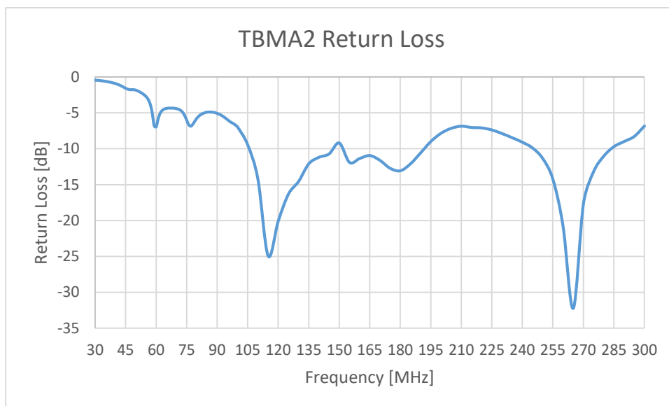
Figure 4: TBMA2 Return Loss 30 MHz ... 300 MHz
