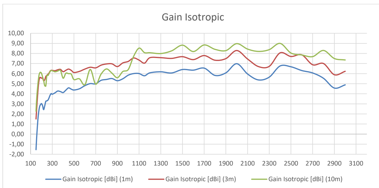
150 MHz ... 3000 MHz, Isotropic Gain of TBMA7
