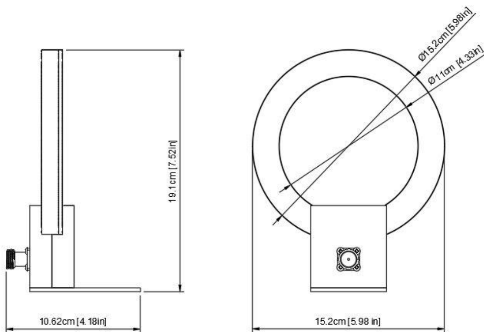
TBRE101 receiving loop dimensions
