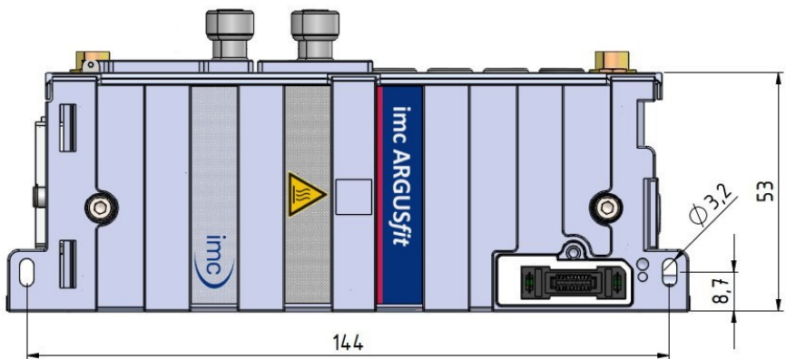
Base unit shown in standard operating position (terminal connections upwards).
