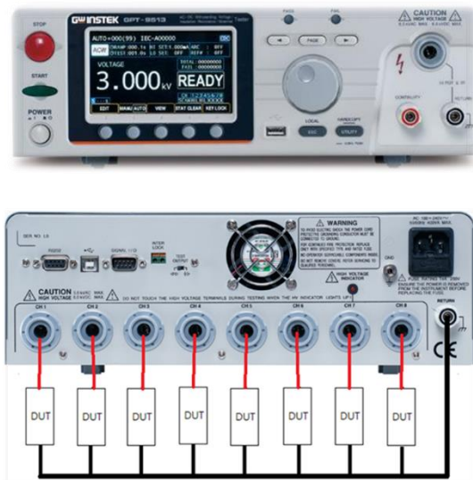
(a) Built-in multi-channel scanner: GPT-9500 series
