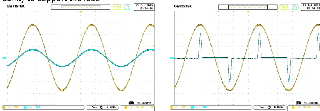
Figure (12) Waveform example of current crest factor
