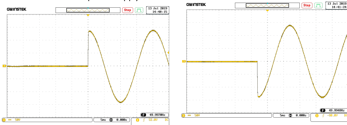
Figure (4) The left picture sets the AC power output to start at 90 degrees, and the right picture sets the output to start at 270 degrees
