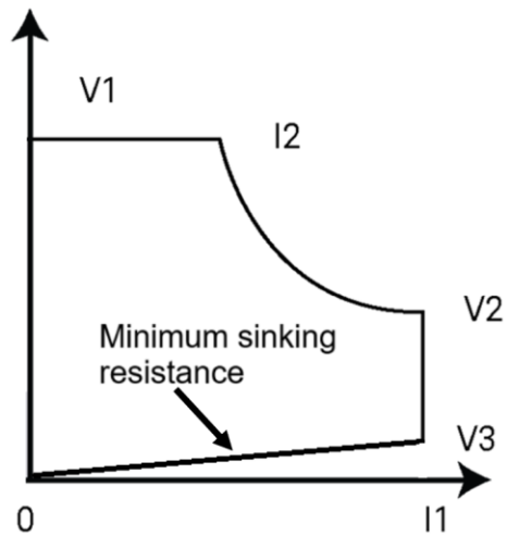
Figure 9. EL4900 characteristic
