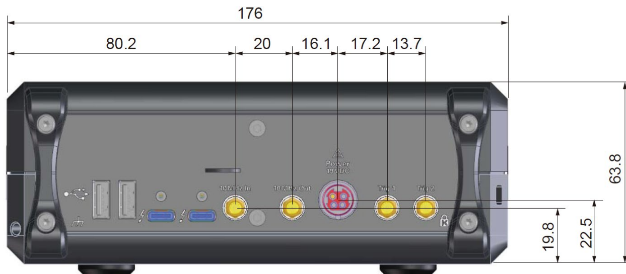
Dimensions (rear view, P5020B/21B/22B/23B/24B/25B/26B/27B/28B with option 400 or 402, or P5020B/21B/22B/23B/24B with option 600, in millimeters)
