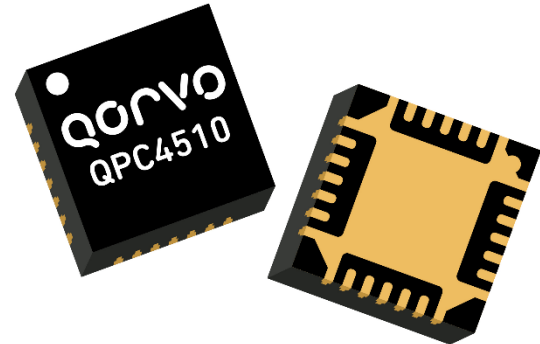
28-pin 5x5 mm QFN package
