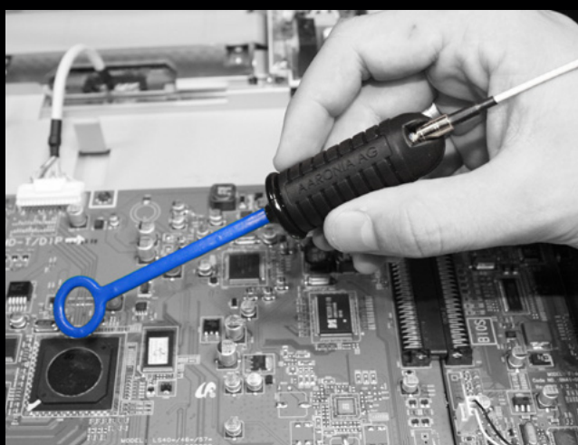
Pinpointing interference sources on a circuit board
