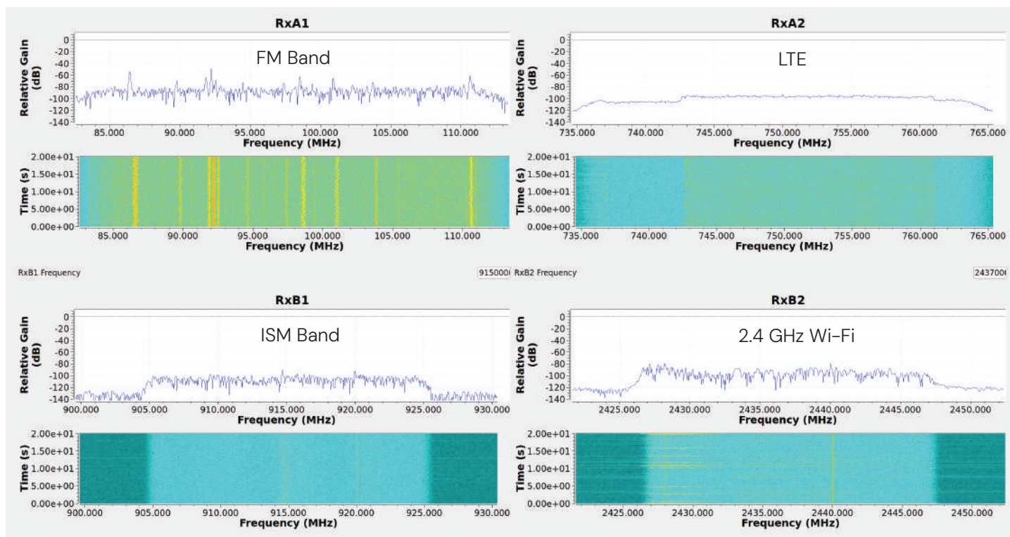
GNU Radio running on the Z4 performing monitoring of four different frequency bands of interest.
