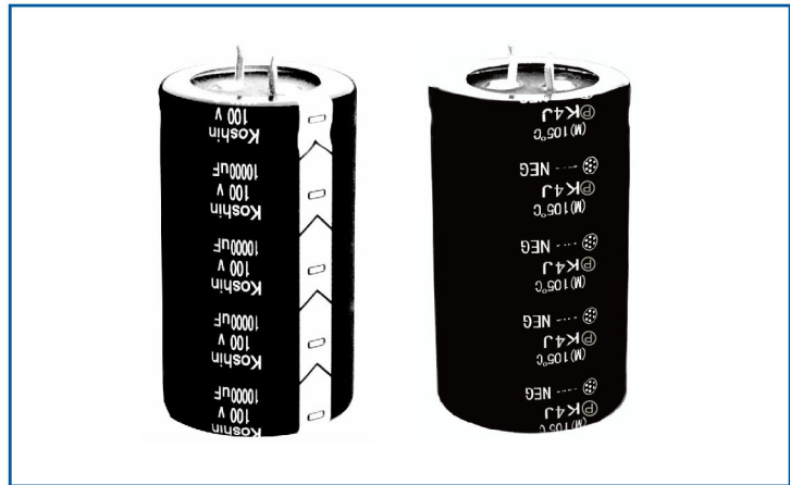
Marking color: White print on black sleeve
