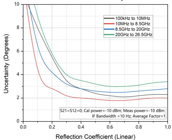
S11 Phase Accuracy
