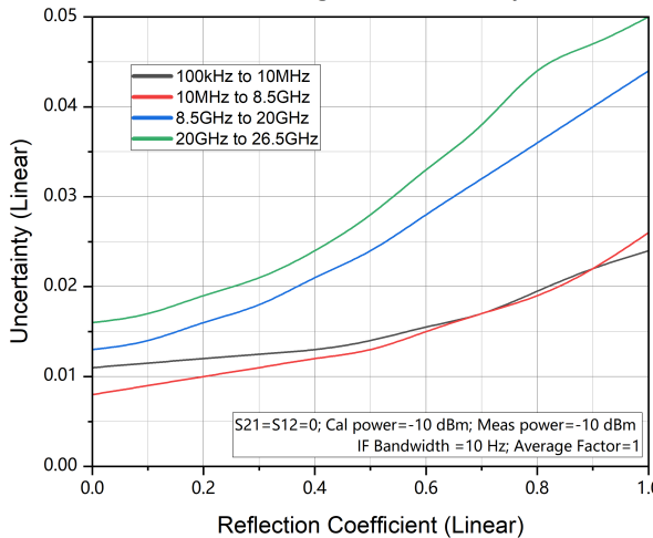
S11 Magnitude Accuracy
