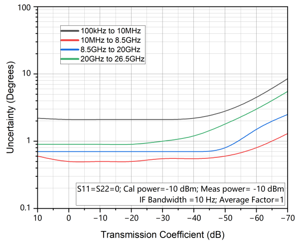
S21 Phase Accuracy
