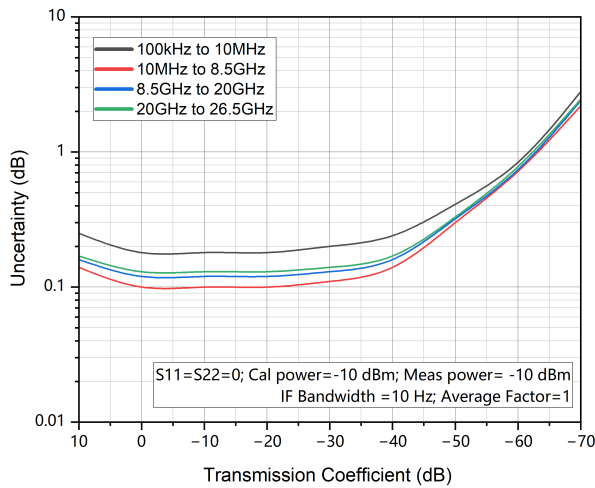
S21 Magnitude Accuracy
