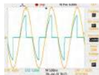
90 Degrees Current Waveforms Leading Edge
