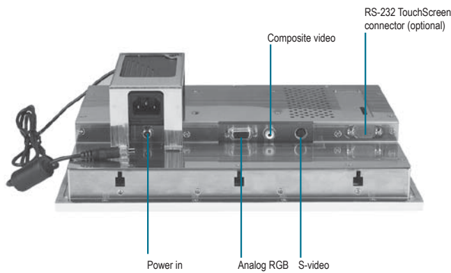
Power in
