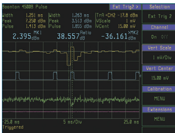
Figure 1: Analysis of CDMA Pulse Train with RF and Trigger Channels Updating Simultaneously
