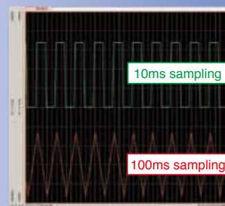
Measurement comparison of 5 Hz square pulse waveform with 10 ms (upper trace) and 100 ms sampling
