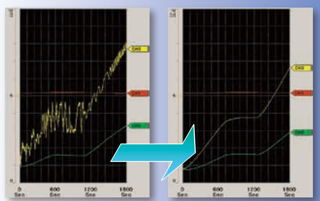
Measurement comparison of abrupt load change in waveform with 10 ms (upper trace) and 100 ms sampling
