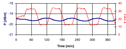
temperature drift of output level
