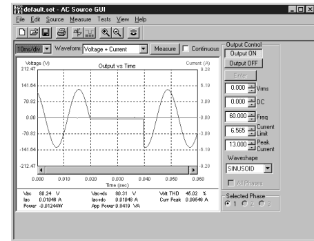
One cycle AC Mains Dropout
