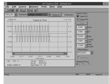
Ringer Voltage (DC + AC) Generation
