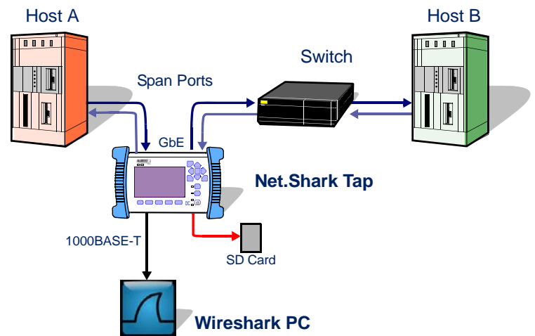
Figure 1. Net.Shark and Wireshark in operation. All-in-one field Tap, Filter, Capture, Aggregation, Regeneration, Drop, Storage, and VNC remote control.
