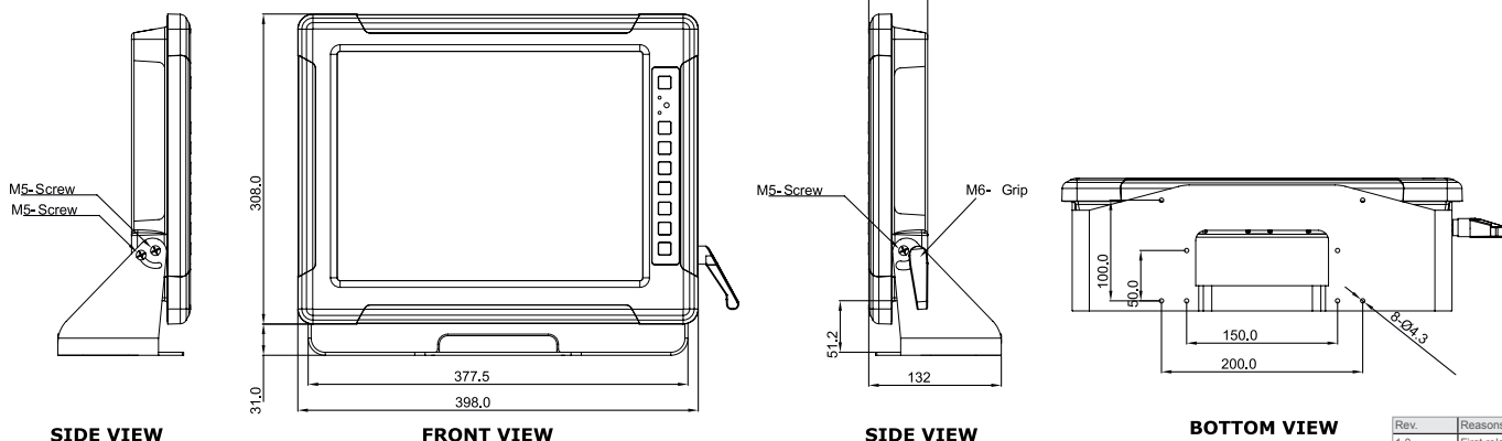
SIDE VIEW
