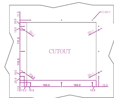
CUT OUT DIMENSION
