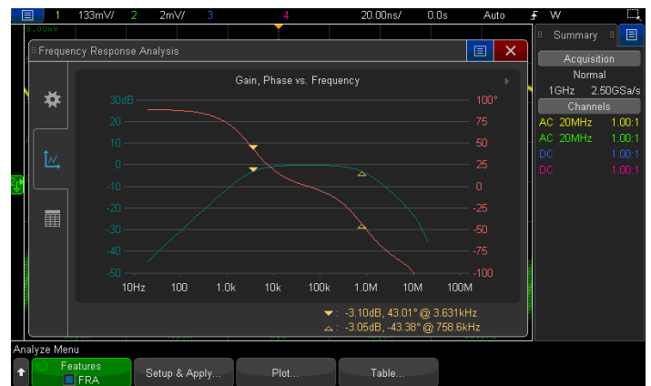
Figure 25. Frequency response analysis plot (Bode gain & phase) of a bandpass filter.
