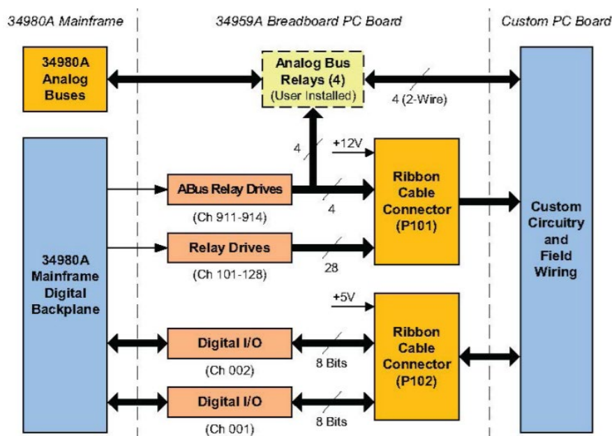
Figure 19: 34959A breadboard module
