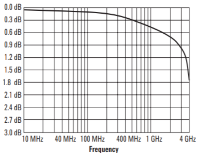
Figure 10: 34941A typical initial insertion loss
