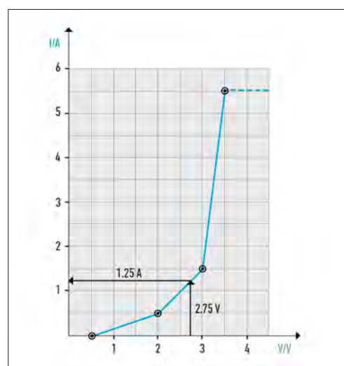
LED characteristic with 4 points
