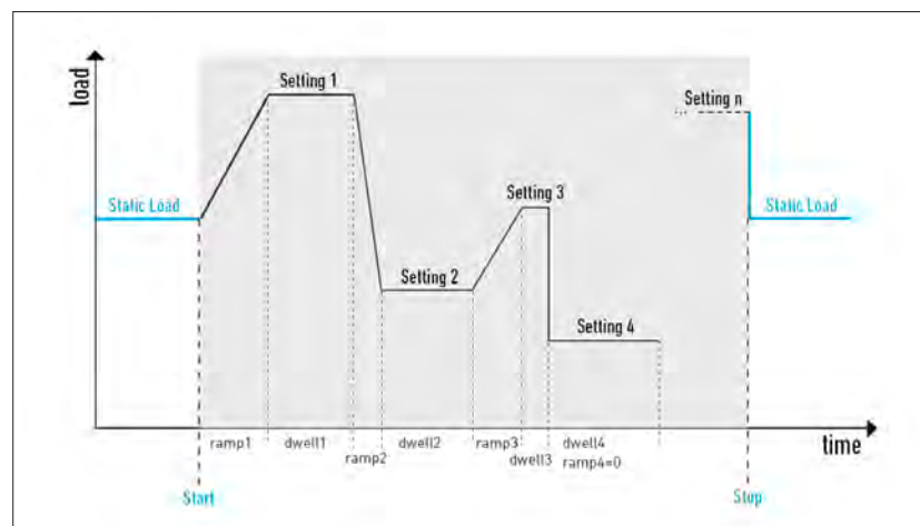
Load profile with LIST function
