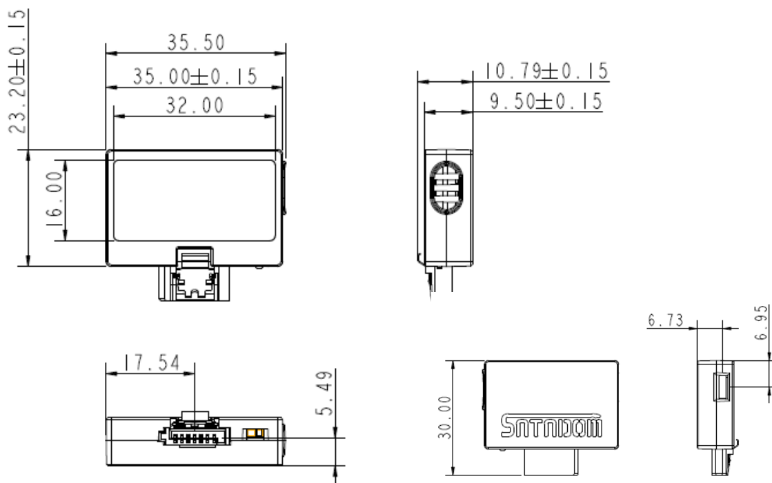
SATADOM D150QV-L mechanical dimensions (* Tolerance is \pm 0.15\text{mm} )
