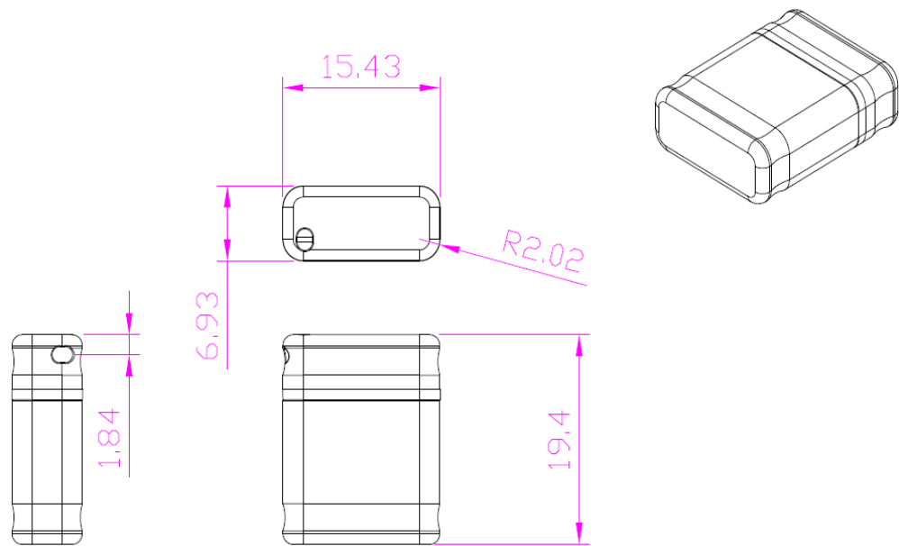
Industrial Nano USB mechanical dimensions (* Tolerance is \pm 0.2\text{mm} )
