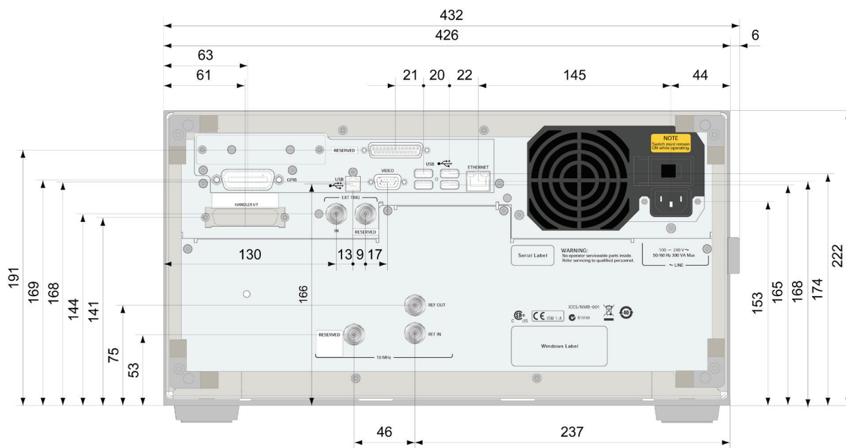
Figure 13. Rear view
