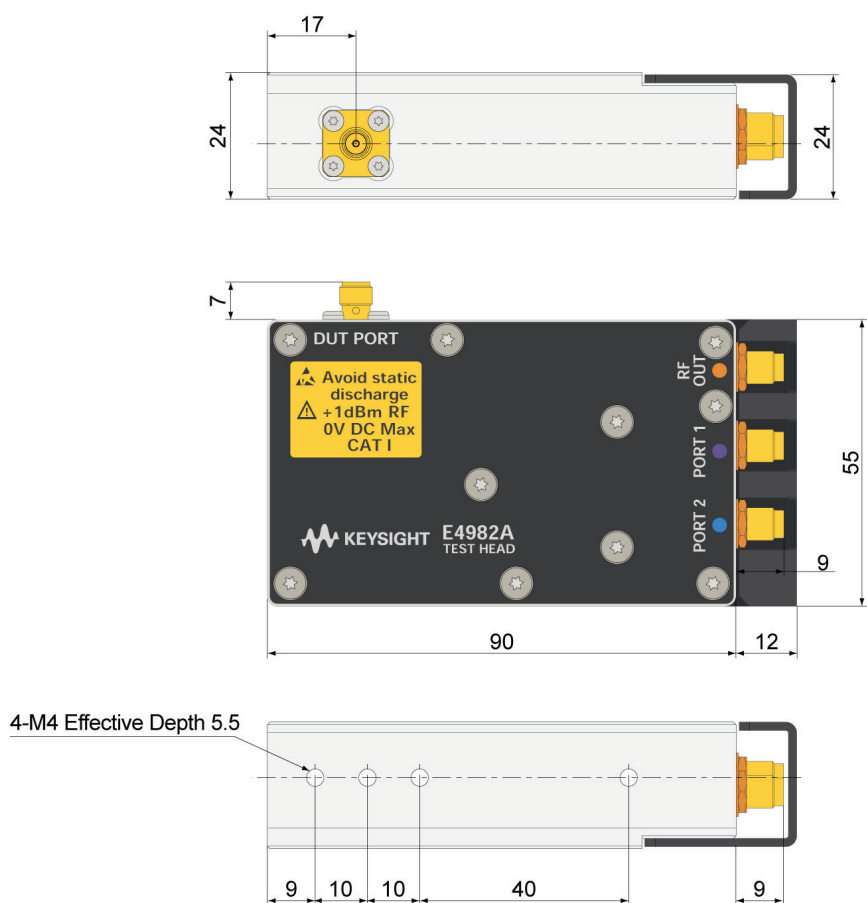
Figure 15. Test head
