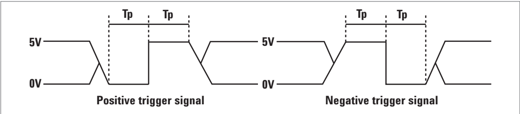
Figure 10. Definition of pulse width (Tp)
