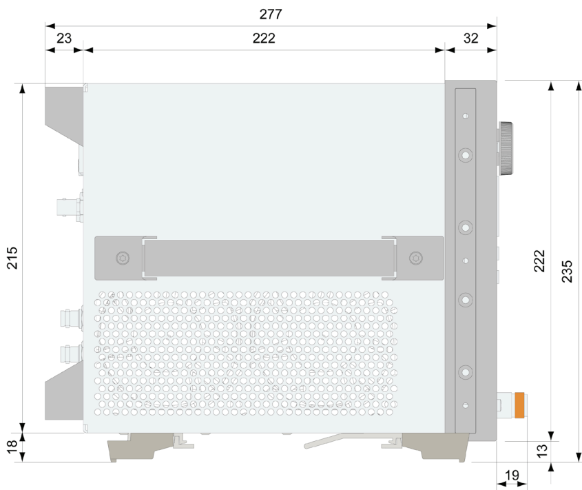
Figure 14. Side view
