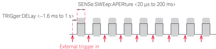
Figure 1. The U2040 X-Series offers real time measurement by measuring every consecutive pulse without dead time.
