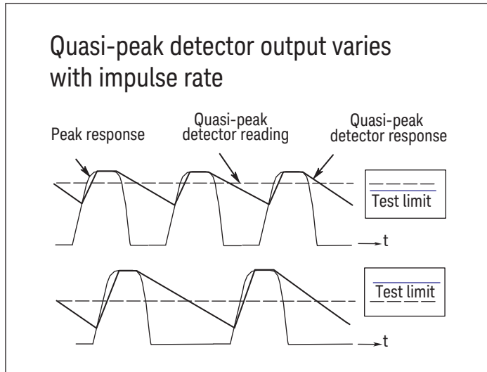
Figure D-2. Quasi-peak detector response diagram
