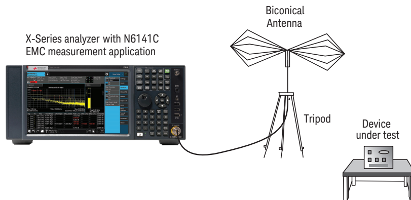
Figure 10. Radiated emissions test setup
