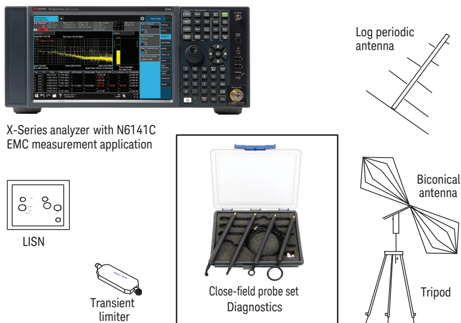
Figure 3. Components of a preproduction evaluation system
