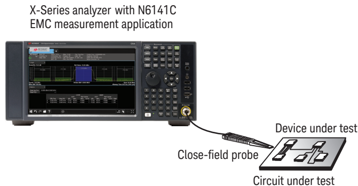
Figure 14. Diagnostics setup interconnection
