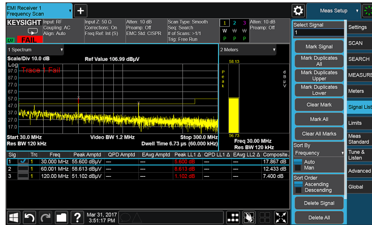
Figure 11. Mark ambient noise and delete it
