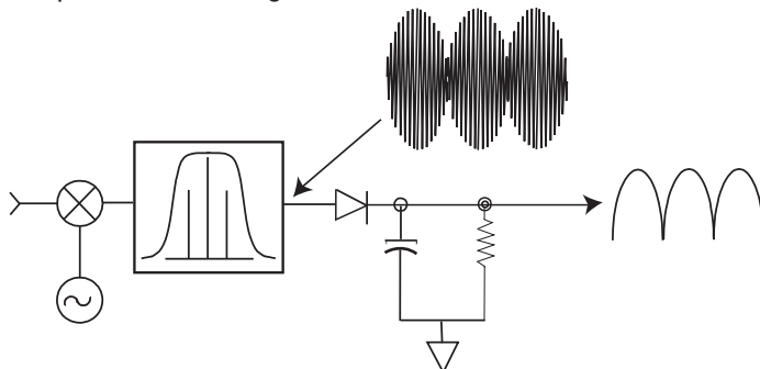
Figure D-1. Peak detector diagram
