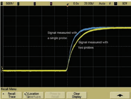
Figure 2-1. Probe loading check with two probes.
