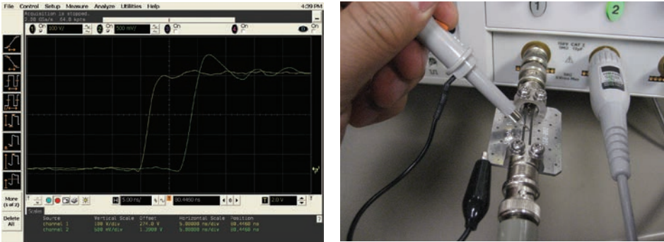
Figure 2-2. Probe loading caused by a long ground lead.
