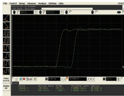
Figure 2-3. Reduced probe loading with short ground lead.
