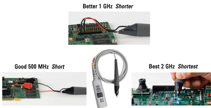
Figure 7. You will achieve higher probe bandwidths with shorter leads.
