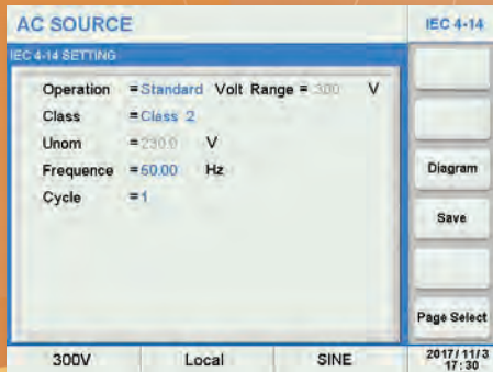
IEC 61000-4-11 Voltage Dip Test Screen - Class 2
