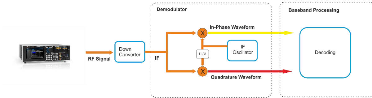
Figure 10: AWG for RF Signals (RX): Arb Rider AWG-4022
