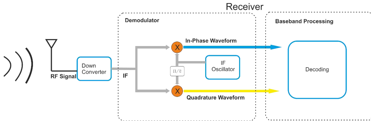
Figure 4: IQ Receiver
