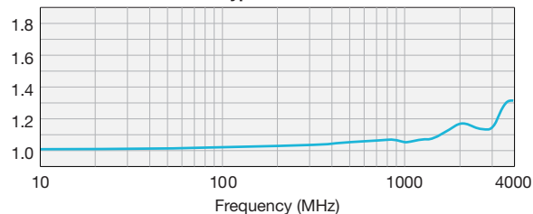
Typical VSWR
