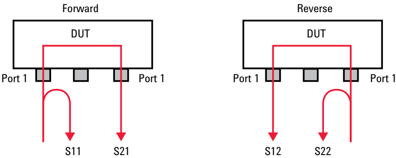
Figure 4. S-parameter definitions for a 2-port device under test (DUT)
