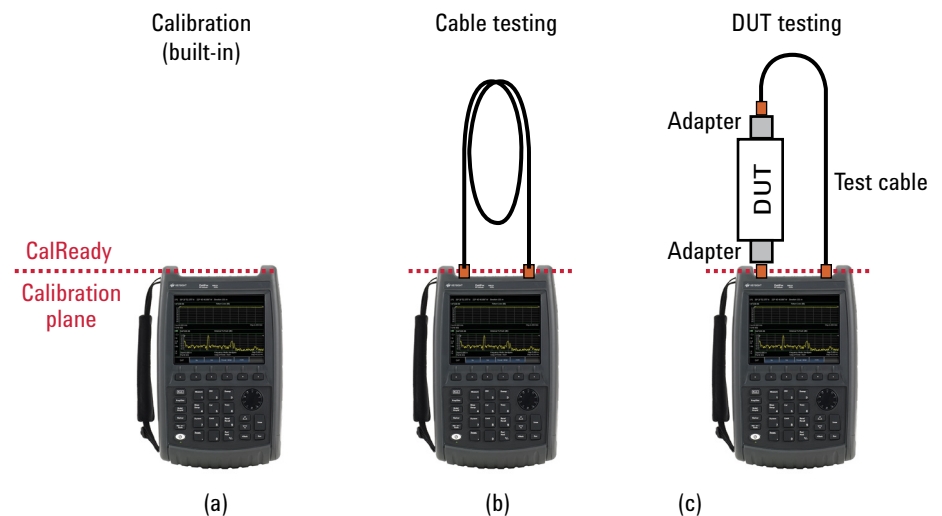
Figure 7. Calibration and test configurations using FieldFox CalReady
