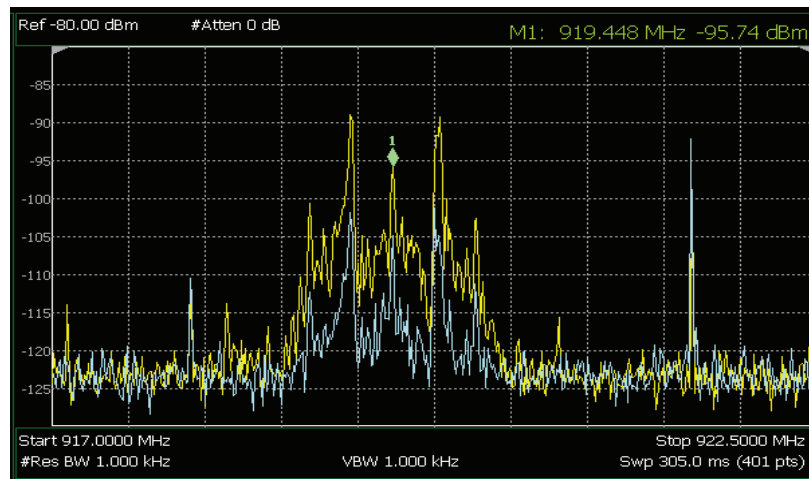
Figure 8. Over-the-air measurement comparing the received signal using an omnidirectional antenna (blue trace) and a high-gain antenna (yellow trace)
