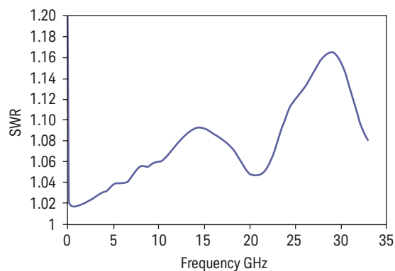
Typical SWR, 10 MHz to 26.5 GHz ( 25 \pm 10^\circ\text{C} ) for N8485A sensor
