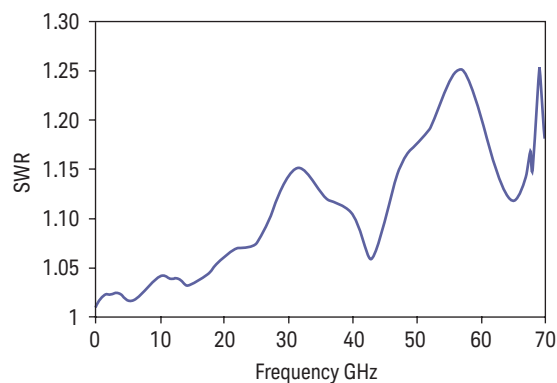
Typical SWR, 10 MHz to 70 GHz ( 25 \pm 10^\circ\text{C} ) for N8488A power sensor
