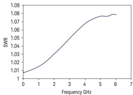
Typical SWR, 100 kHz to 6 GHz (25 ±10°C) for N8482H power sensor
