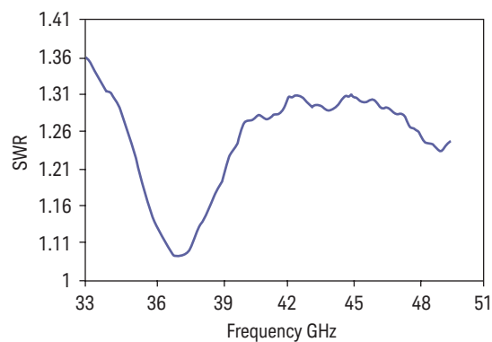
Typical SWR, 33 to 50 GHz ( 25 \pm 10^\circ\text{C} ) for N8486AQ power sensor
