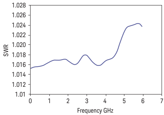
Typical SWR, 100 kHz to 6 GHz (25 ±10°C) for N8482B power sensor
