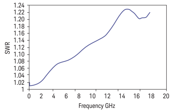
Typical SWR, 10 MHz to 18 GHz (25 ±10°C) for N8481H power sensor
