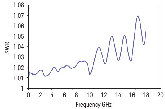
Typical SWR, 10 MHz to 18 GHz (25 ±10°C) for N8481B power sensor
