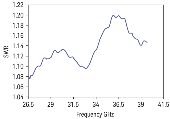
Typical SWR, 26.5 to 40 GHz (25 ±10°C) for N8486AR power sensor
