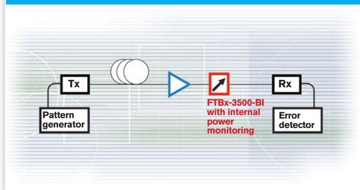
Figure 2. Typical receiver sensitivity setup
