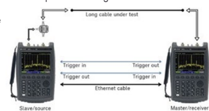
Measure long, lossy cables using ERTA
