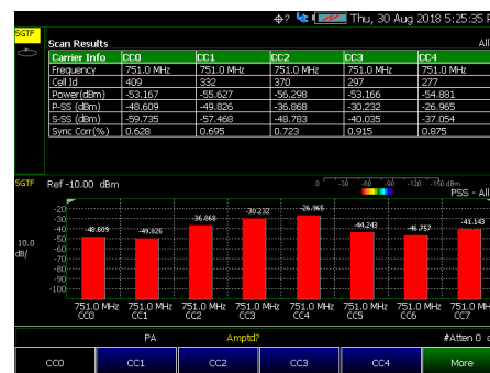
5G TF OTA measures control channels and displays cell ID
