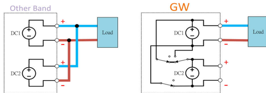
Output in parallel connections
