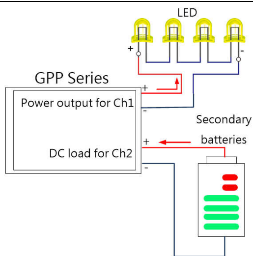
GPP series application
