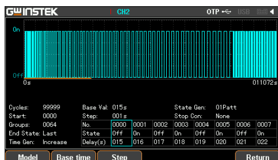
GPP series delayed waveform
