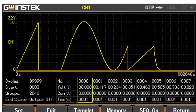
Output waveform of the GPP series
