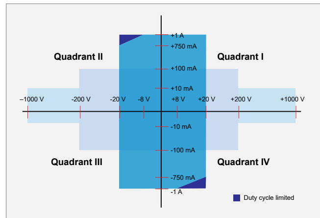
2470 power envelope.
